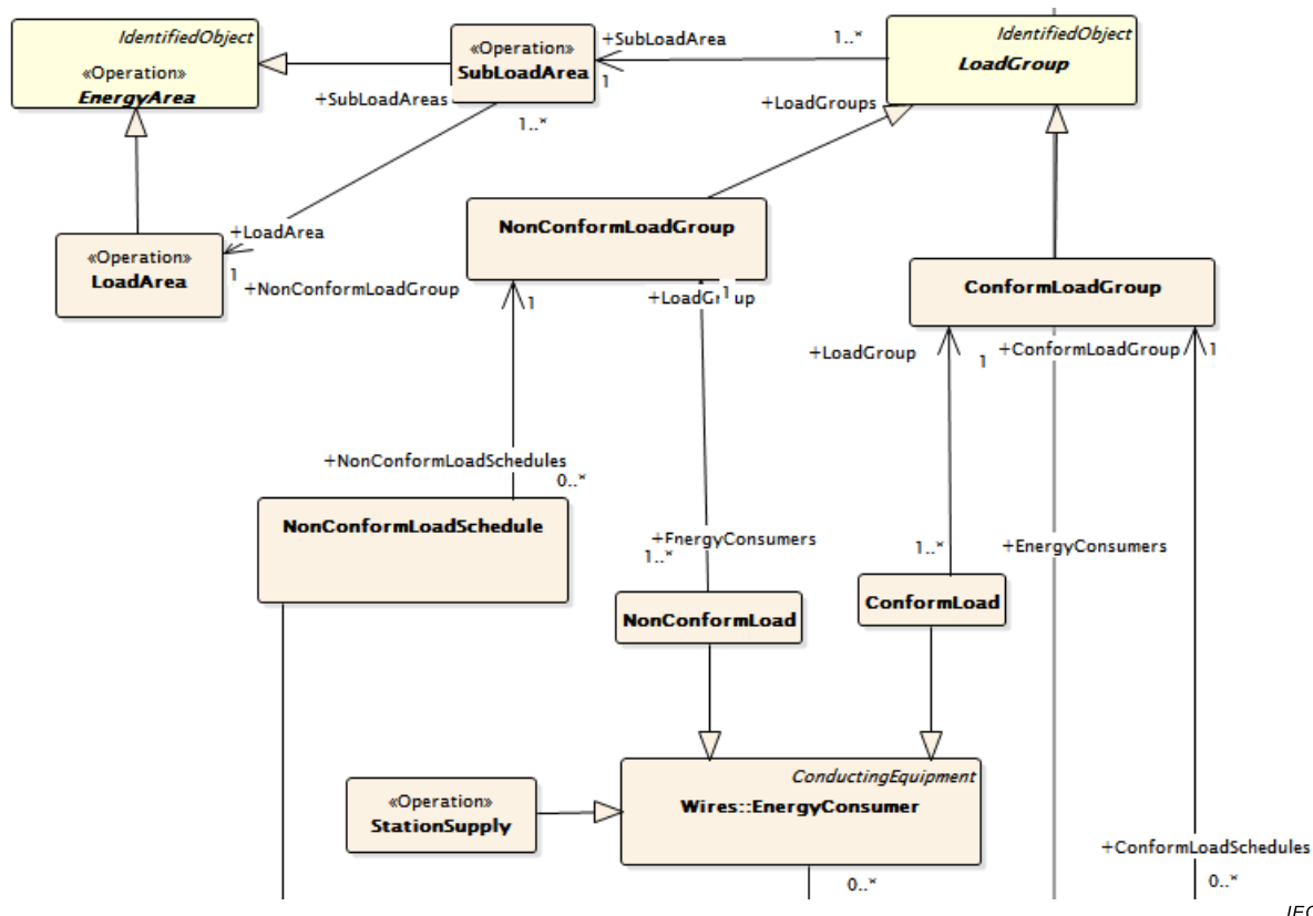
Figure E.1 – Diagram ConformLoadGroup/NonConformLoadGroup
