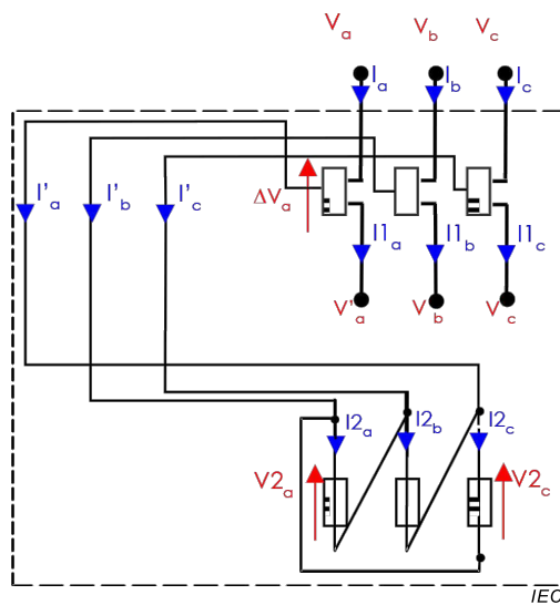
Figure D.3 – Dual core and single core
