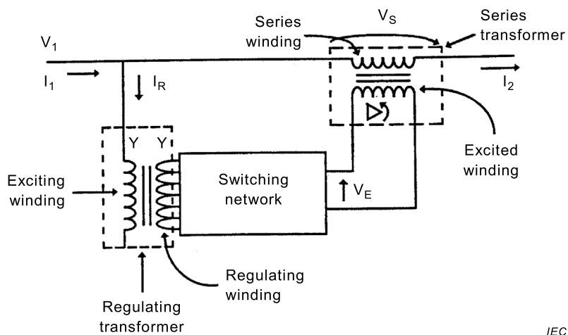
Figure D.19 – Asymmetrical phase shifter with two cores
