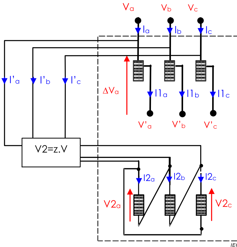
Figure D.22 – Asymmetrical phase shifter with a single core
