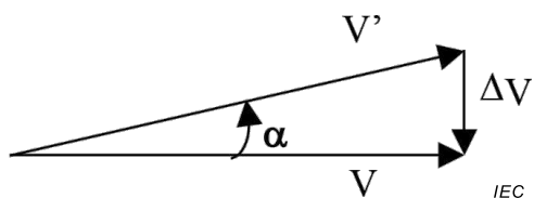
Figure D.18 – Phasor diagram
