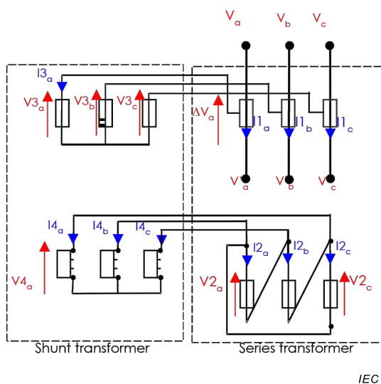
Figure D.3 – Dual core and single core
