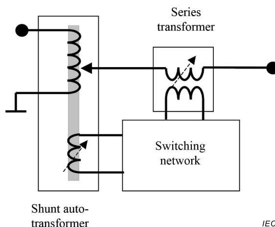
Figure D.11 – In-phase regulating auto-transformer
