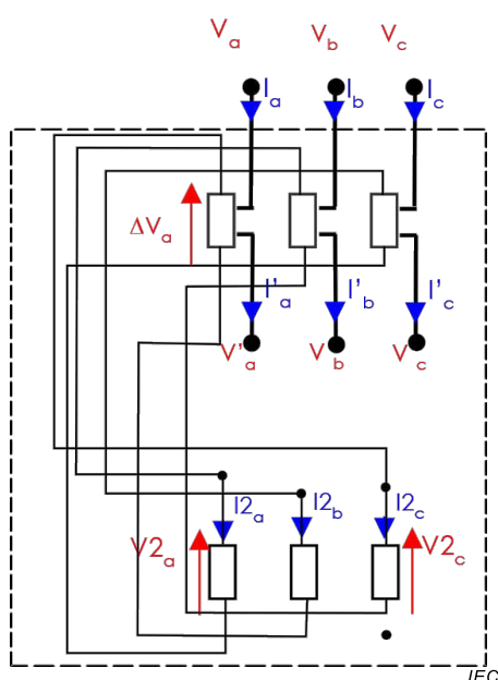
Figure D.4 – Single core, delta hexagonal
