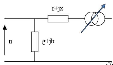
Figure E.3 – Power transformer modelling
