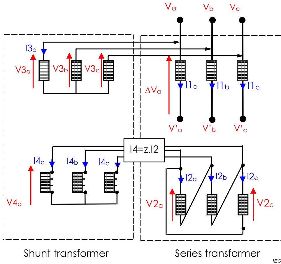
Figure D.20 – Detailed three phase diagram
