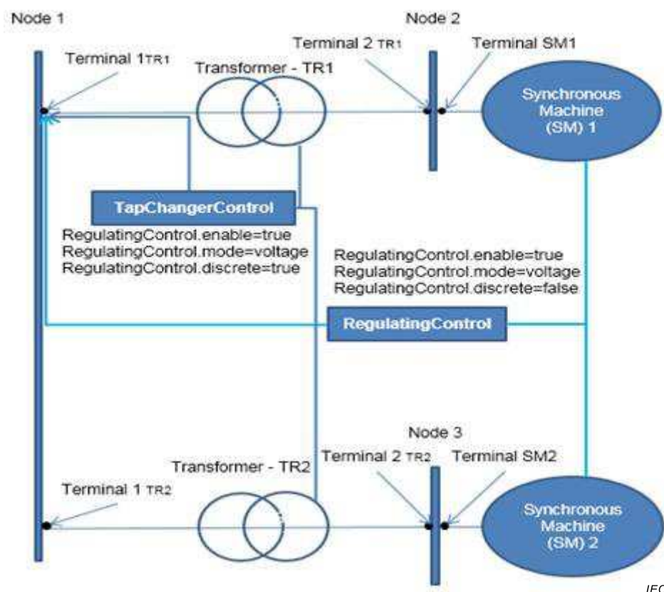
Figure E.2 – Regulating control setup
